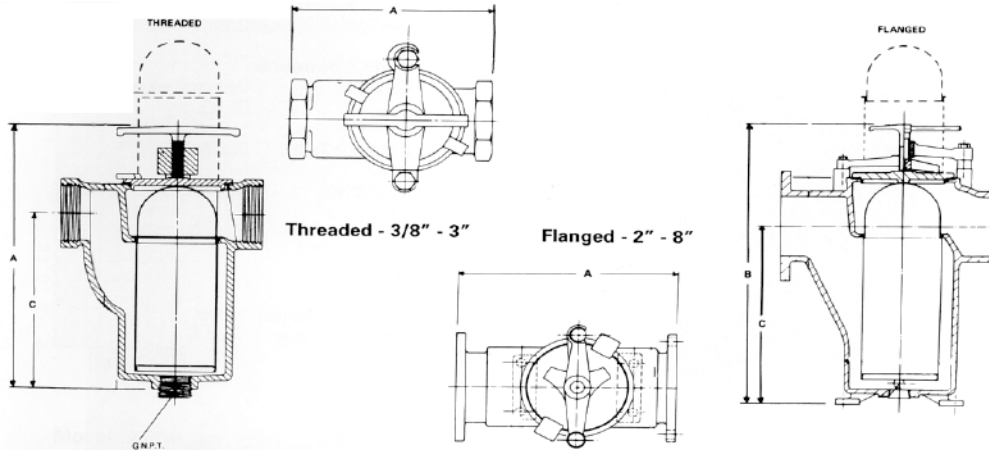
Model 72 Simplex Pipeline Strainer.
